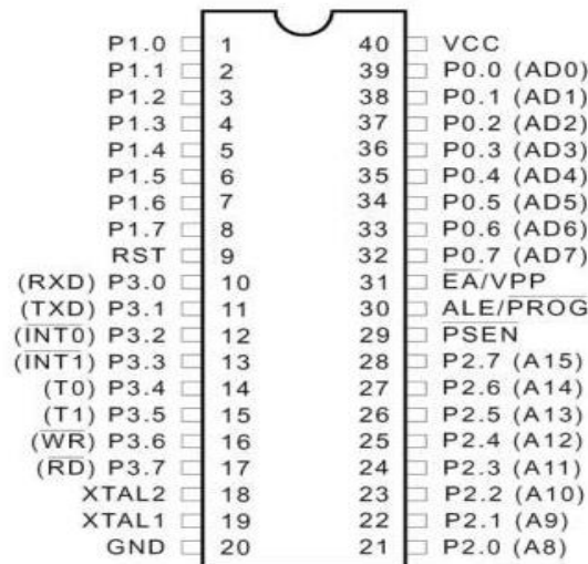
Fig 8: Pin details of AT89C51
