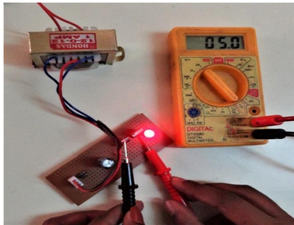
Fig 3: Power supply circuit showing an output voltage of 12.3V and 5V DC from a input of 240V, 50 Hz AC supply
