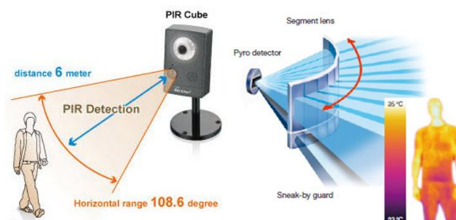
Fig 7: Working of PIR Sensor
