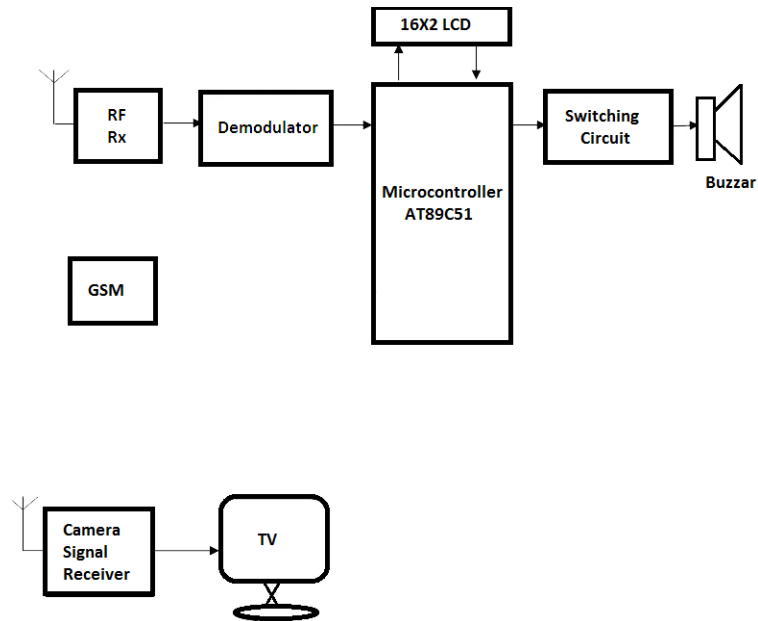
Fig 2: Block Diagram of Controlling Station
