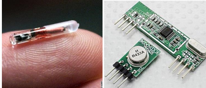
Fig 4: RFID tag and RF transmitter-receiver module containing the integrated antenna and microchip
