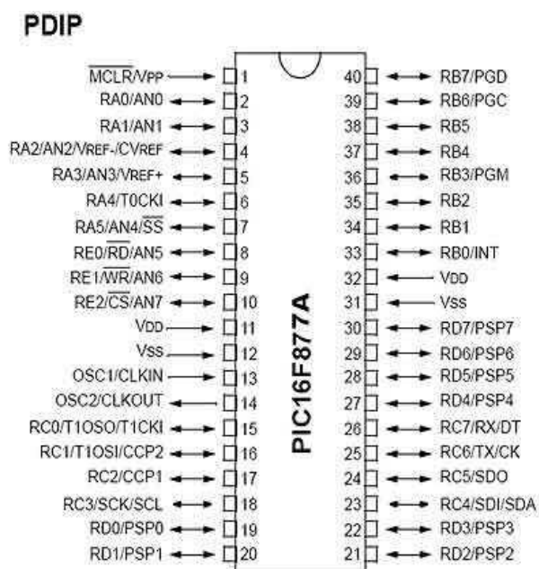
Fig 9: Pin details of PC16F877A
