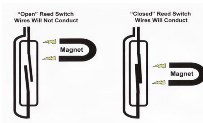
Fig 10: Reed switch sensor operation
