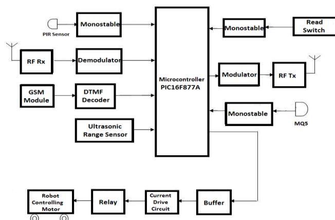
Fig 1: Block Diagram of UMRV
