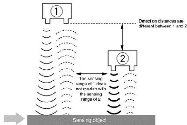
Fig 6: Basic illustration showing how the ultrasonic range finder works
